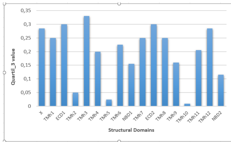
FIGURE 3. Histogram of Quartil_3 values for each structural domain. Every bin represents a structural region; TMDs are divided into different TMhelices (TMhs). X domain represents the residual, not structured portion of the ABCA4 sequence.
