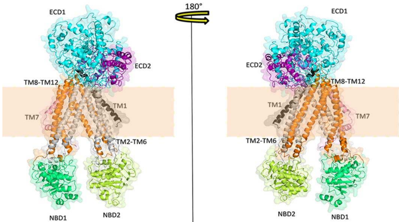
FIGURE 4. Surface and cartoon representation of human ABCA4 3D structural model overview. Human ABCA4 structure is reported in surface and cartoon representation. The TM1, ECD1, TM2-TM6, NBD1, ECD2, TM7, TM8-TM12, and NBD2 domains are labeled accordingly. The TM regions are depicted with dotted lines.
